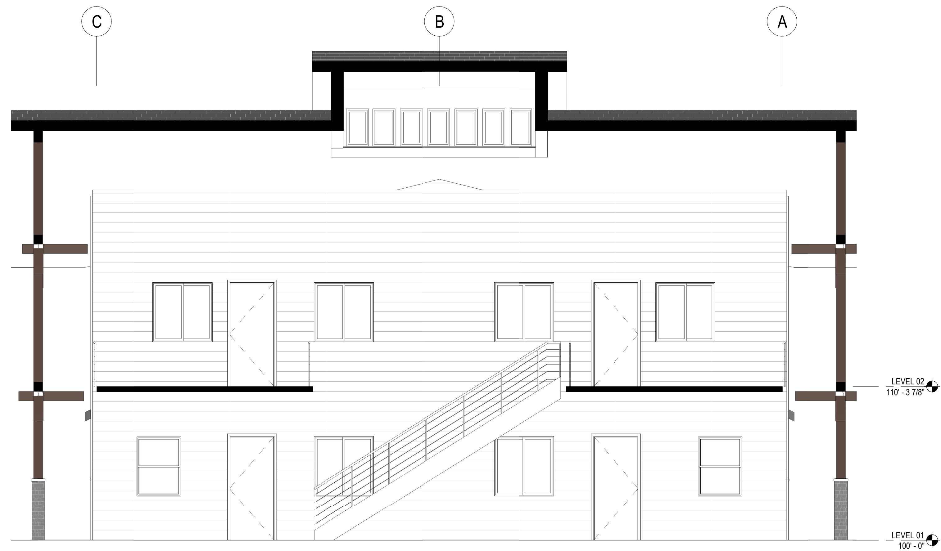
C1 EXTERIOR ELEVATION - INSIDE 1/4" = 1'-0"
